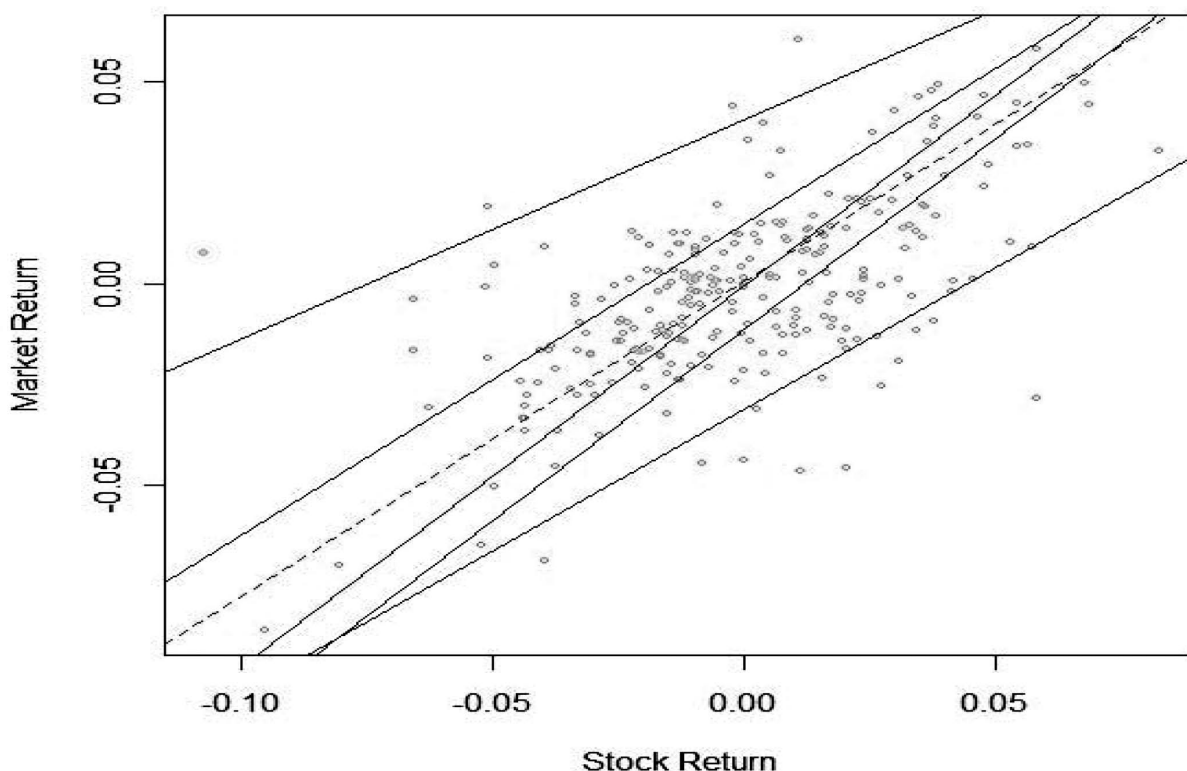
FIGURE 1: Scatter and quantile regression fit to the return data of stock (QBE Insurance)
