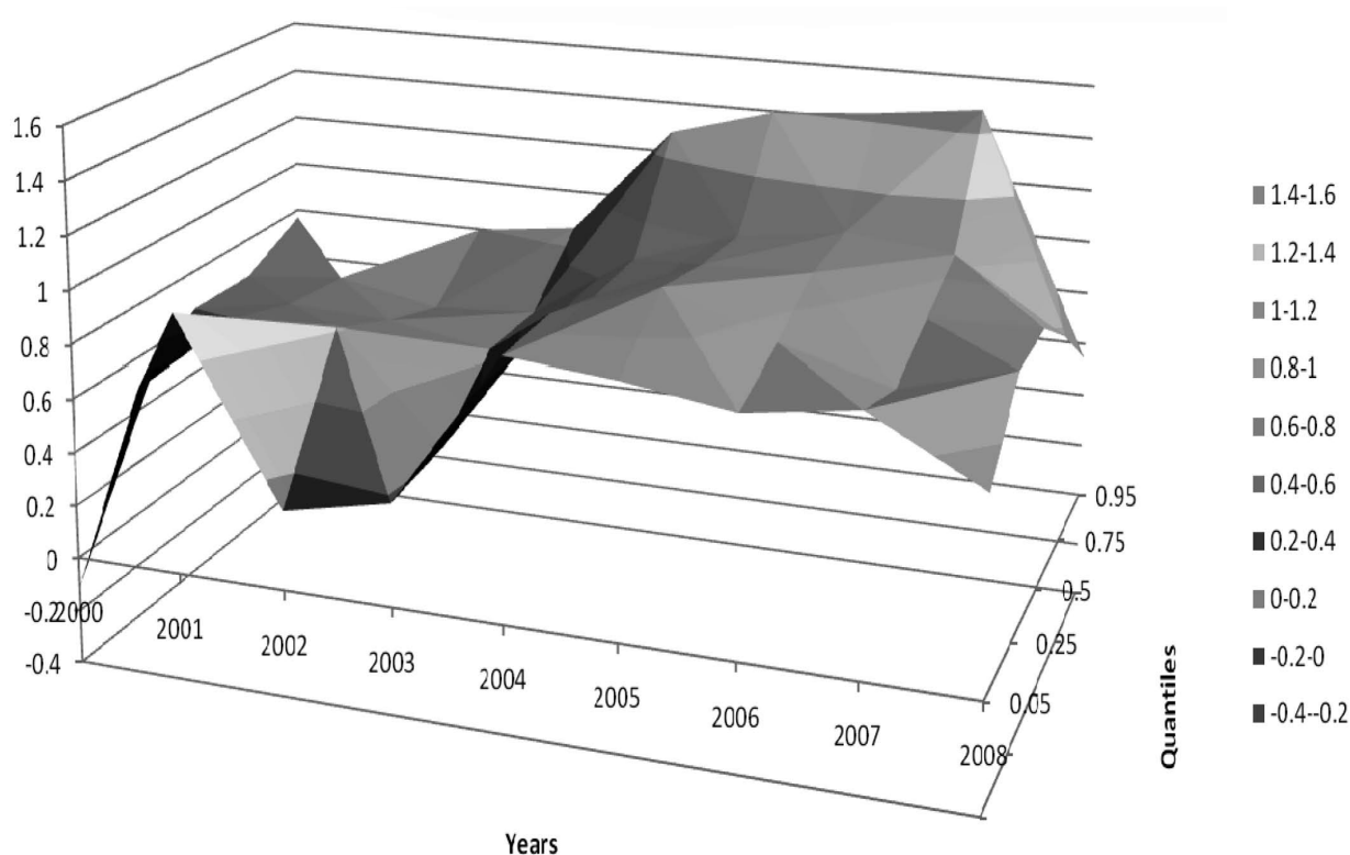
FIGURE 3: Beta values across quantiles each year
