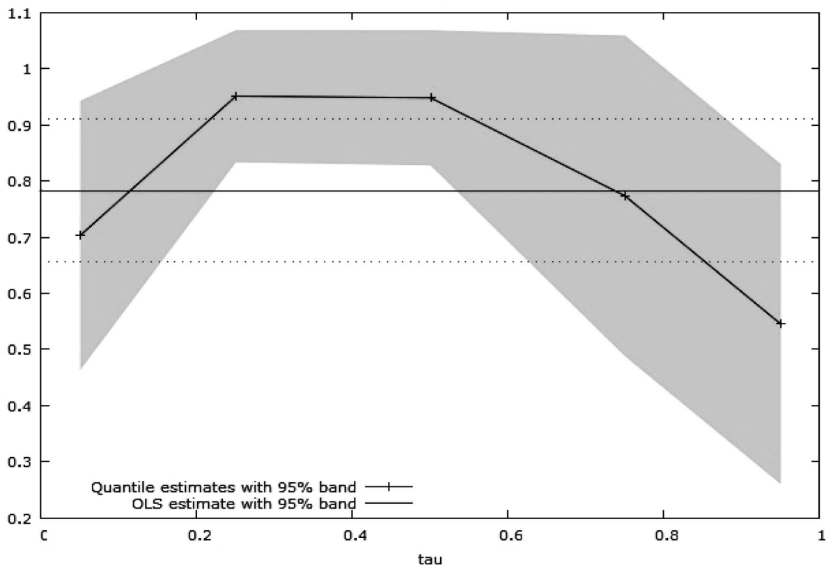
FIGURE 2: Beta values across quantiles and OLS for stock (QBE Insurance)
